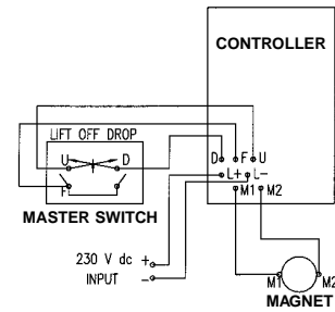
SYSTEMS DIAGRAM
